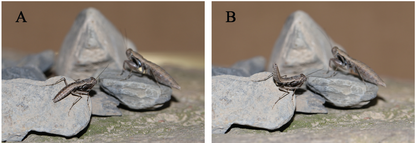
Fig. 1. Orientation of male Holaptilon brevipugilis abdomen in a frontal encounter with a female prior to copulation. A. Plantar flexion and B. Dorsiflexion of the abdomen. The male is in the foreground on the left and the female is to the rear and to the right of the male.
